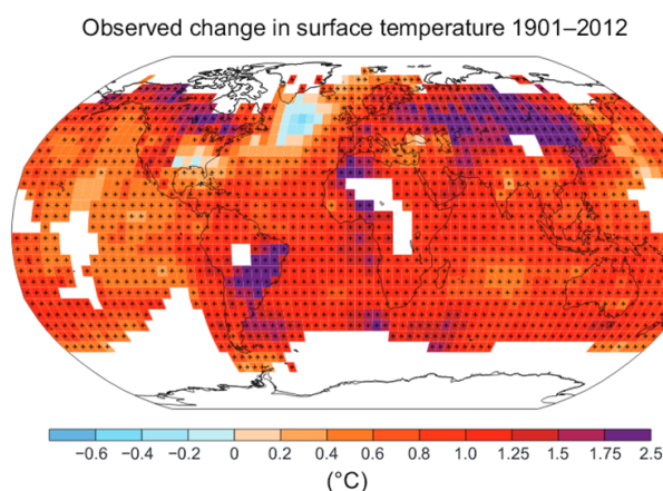
Figure 15. Map showing changes in surface temperature (IPCC AR5 WG1 Figure SPM.1b p.6 [44]).
