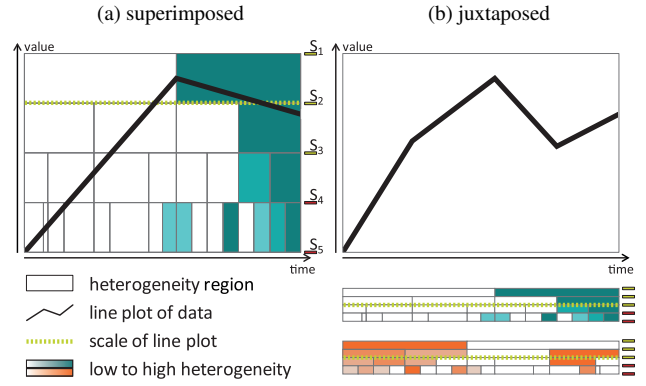
Figure 3: The principle design of our visualization approach: Heterogeneity bands are stacked and visualized either behind (a) or next to the data (b). In both cases, saturated colors indicate changes between the data of subsequent scales. The green dashed horizontal cursor indicates the scale of the currently visualized trajectory and the small colored bars to the right show, if the data plot of a scale is affected by overplotting (red) or not (green).
