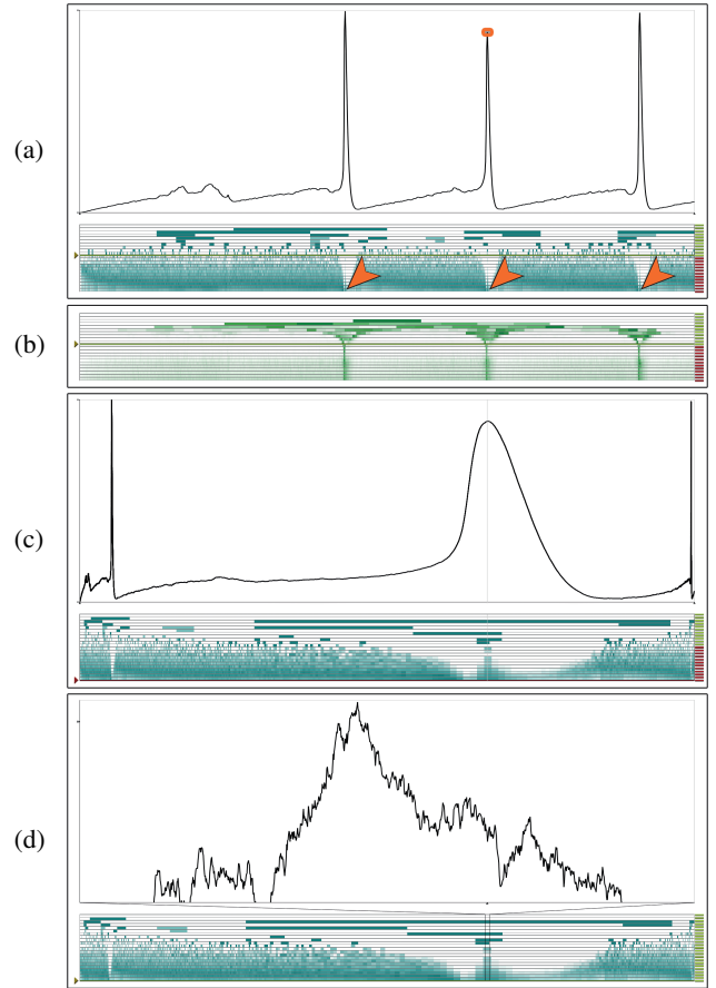
Figure 7: Trajectory of MPF_a from a simulation with k_d = 3 and dynamic cell volume (a). Our slope-based metric reveals an uneven distribution of heterogeneities for finer grains with heterogeneities at the peaks (arrows). A metric sensitive to value changes reveals a clear differentiation from surrounding areas at those scales (b). Applying a fisheye lens preserves a distorted overview (c). Only a drill-down to the finest grain and following magnification at those areas reveal fluctuation at the top of a peak (d).
