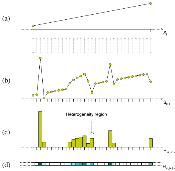
Figure 1: To determine heterogeneities between subsequent scales S_i and S_{i+1} we simply map the data points of one scale at the respective other scale (a, b). The calculated heterogeneity values are aggregated into heterogeneity regions of principally arbitrary size (c). To provide intrascale guidance, we choose the grain of S_{i+1} as the regions' size. A compact representation is gained by so called heterogeneity bands mapping heterogeneities to color (d).
