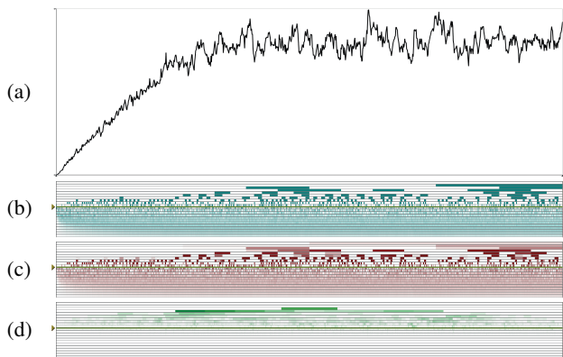
Figure 6: Trajectory of MPF_a from a simulation with k_4 = 2 \text{ min}^{-1} , i.e., k_d = 2 \text{ min}^{-1} and the cell volume V = 1 is constant (a). Our metric reveals equally distributed changes in slope throughout the whole trajectory (b) suggesting the existence of noise. A second metric quantifying slope changes bares the same behavior (c). A third metric (d), which is sensitive to value changes, reveals only marginal changes at more fine-grained scales.
