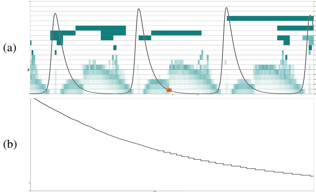
Figure 4: Within a simulation time series, a repeating pattern at the more fine-grained scales attracts attention (a) and unveils a faulty switch within the simulator’s behavior (orange box enlarged in b).
