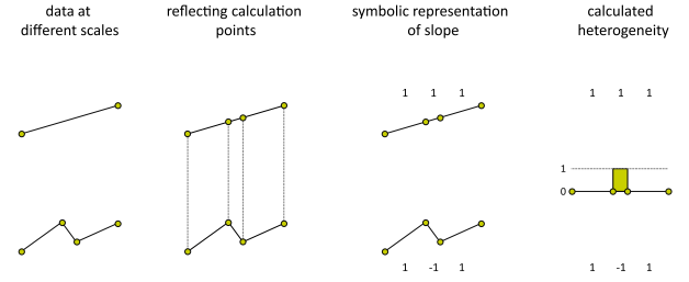
Figure 2: Our metric detects changes in the slope between subsequent scales. If slopes of subsequent scales differ in their direction, a heterogeneity value of 1 is assigned – otherwise 0.
