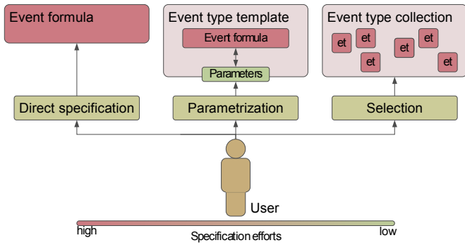
Fig. 15. User-centered event specification model – Event types can be specified by using event formulas directly (left), by parameterizing event type templates (middle), or by selecting from a predefined application-specific collection of event types (right). The effort required for event specification decreases in the same order.
