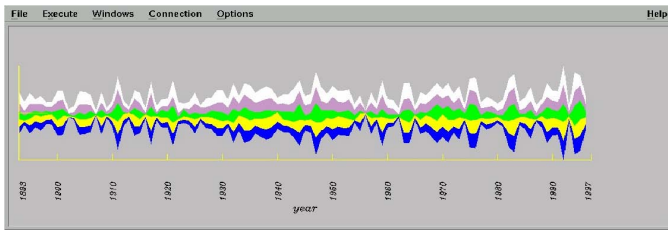
Fig. 10. Visualization of a climate dataset using a ThemeRiver [32] approach. The graph depicts five time-dependent variables: summer warmth (blue), summer days (violet), hot days (green), summer mean temperature (yellow), and mean of extreme (white) for a period of more than 100 years.
