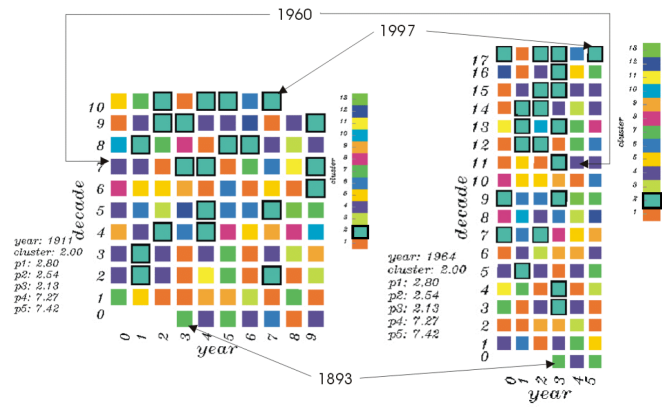
Fig. 13. Rectangular View – Visualization of a temporal clustering of meteorological time-oriented data from the Potsdam observation station. Thirteen clusters of yearly temperature curves have been extracted from the data. In this example, changing the periodicity (denoted as decade) from 10 years (left) to 6 years (right) helps in identifying a temporal pattern for cluster 2 (see [37]).
