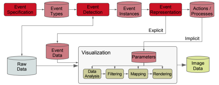
Fig. 14. Model of event-based visualization – The figure shows the major steps of event-based visualization (event specification, event detection, and event representation) attached to the well-known visualization pipeline.
