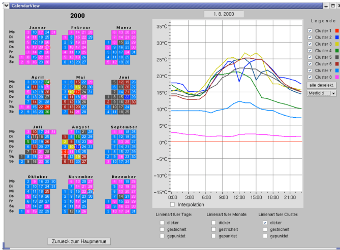
Fig. 12. Cluster Calendar View [36], [37] – The plots show cluster representatives as daily temperature profiles. The calendar view illustrates by color which days belong to which cluster, i.e., show similar profiles.
