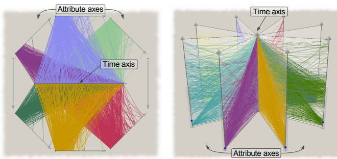
Fig. 2. TimeWheel – Multivariate time-oriented data represented using a TimeWheel – left: a 2D TimeWheel [12], right: the 3D analog [13].
