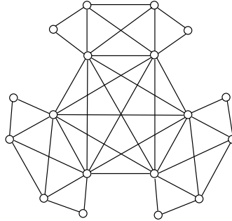
Figure 1: A directed path graph which is not tree 3-spanner admissible
